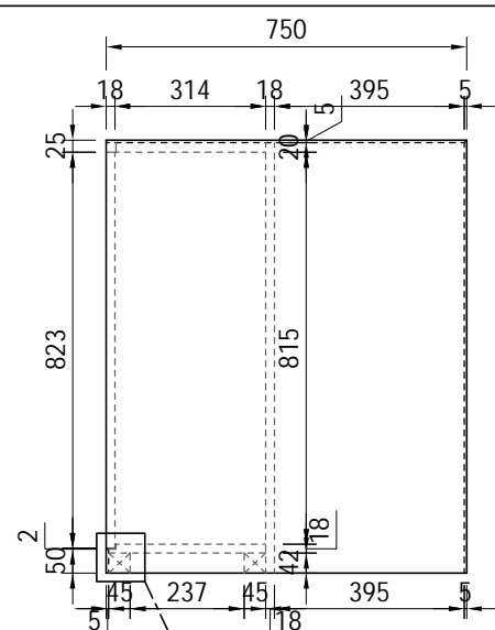
③ Side View 侧立面视图
