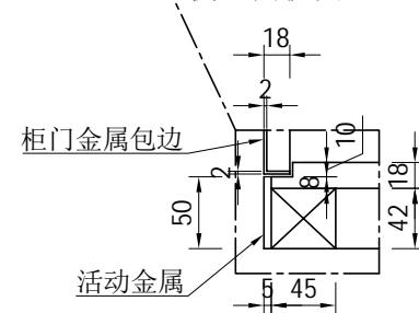
③ Side View 侧立面视图
